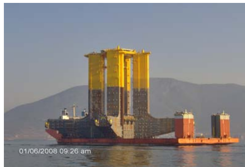
Dry Transportation of Shenzi Hull from Korea to GoM
